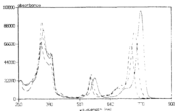
Fig. 3. Quantitative absorption spectra of bacteriochlorophylls, modified at position 3 in diethylether: BChl a (1), (—); [3- \alpha -hydroxy-ethyl]-BChl a (4), (---) and [3-vinyl]-BChl a (7), (- · - ·).
