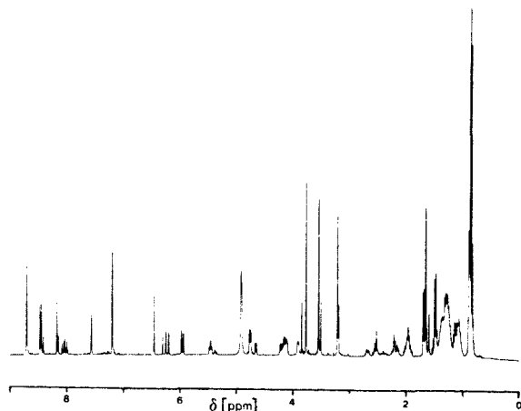
Fig. 1. ^1\text{H} NMR spectrum of [3-vinyl]-BChl a (7) ( 13^2 -epimer mixture) in pyridine- d_5 . Solvent signals at 7.2, 7.56 and 8.69 ppm (pyridine) and at 4.88 ppm (water).
